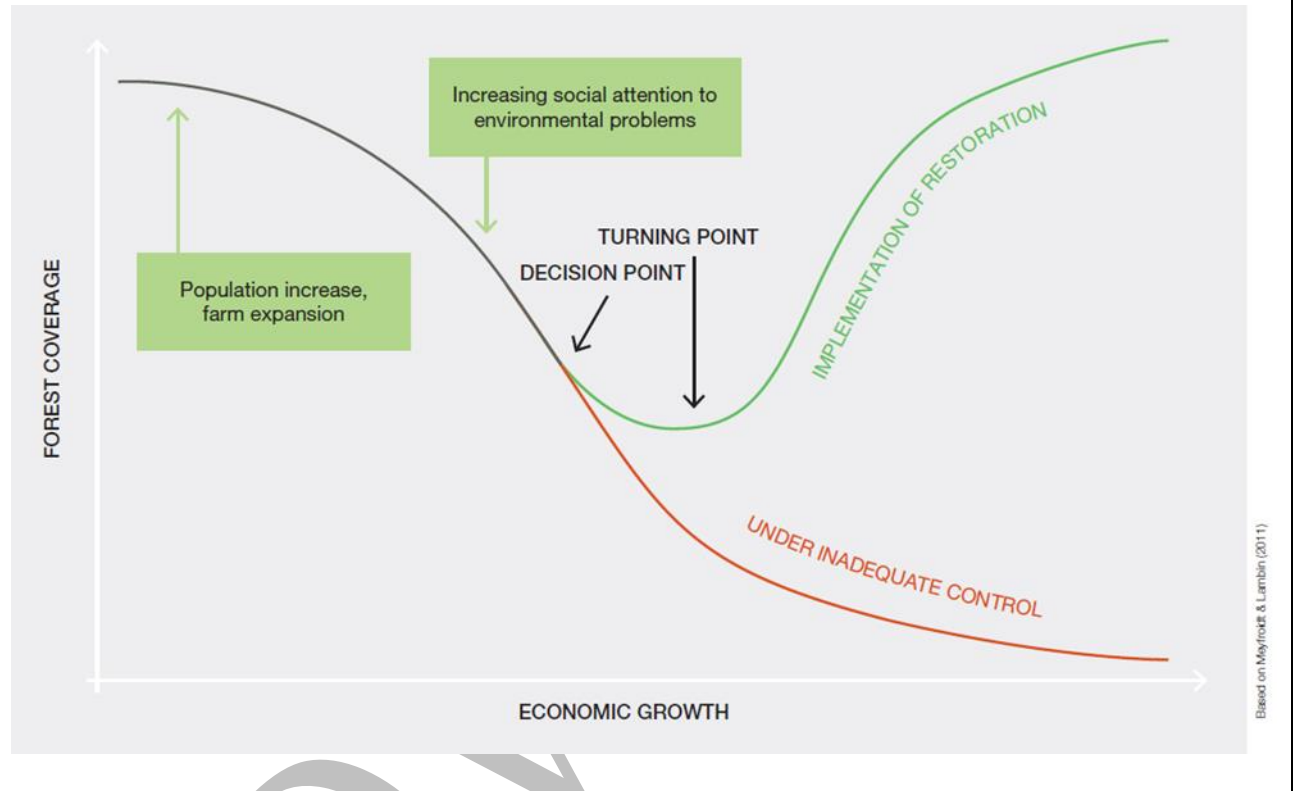
Figure SPM.3
